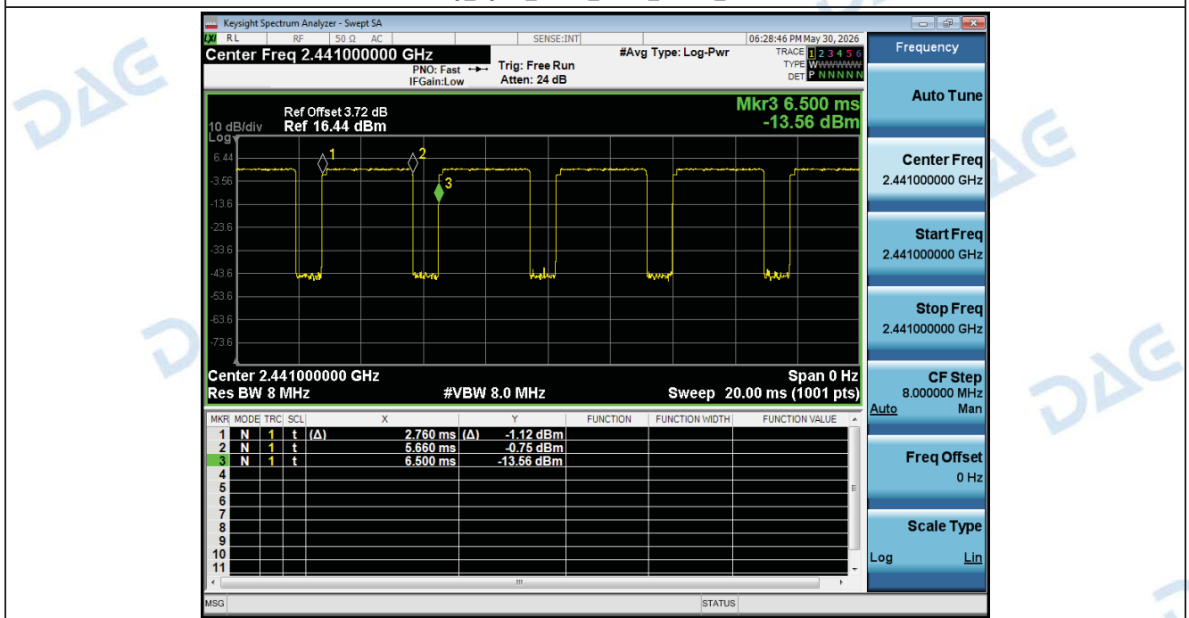
Duty_Cycle_NVNT_ANT1_2-DH5_2441
