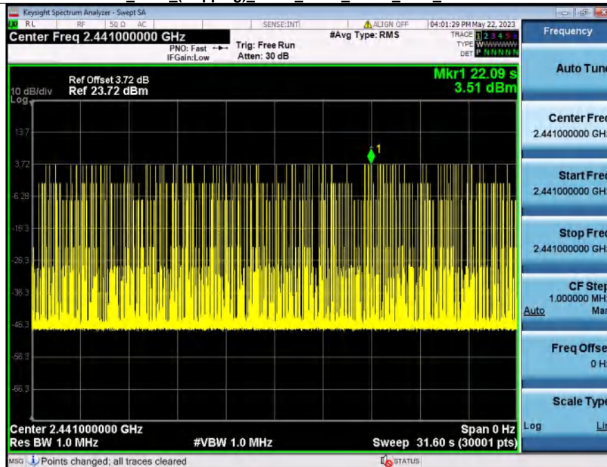
Dwell_Time_(Hopping)_NVNT_ANT1_1-DH5_2441_Accumulated
