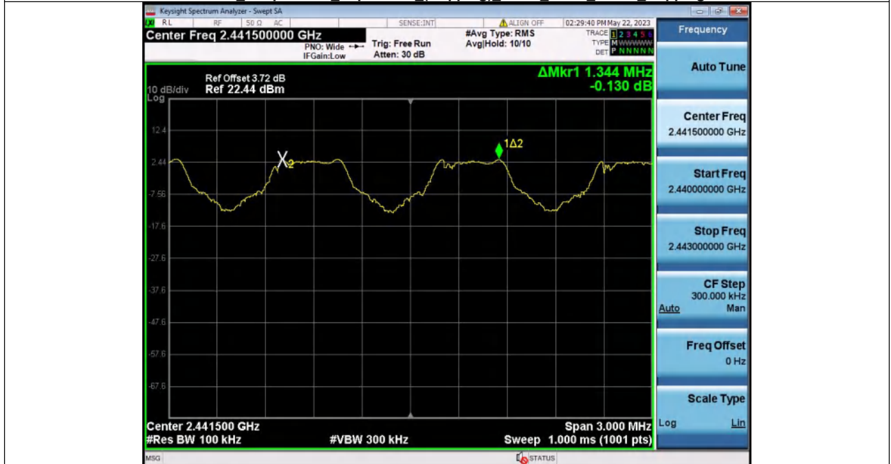
Carrier_Frequencies_Separation_(Hopping)_NVNT_ANT1_1-DH5_Hopping
