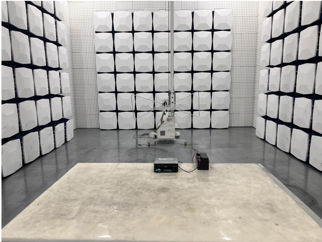
RADIATED EMISSION MEASUREMENT (below 1G)
