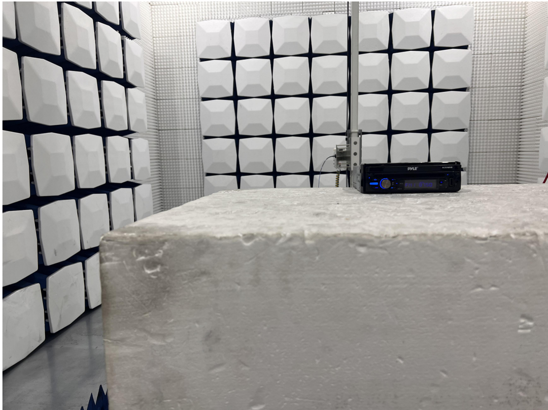
RADIATED EMISSION MEASUREMENT (Above 1G)
