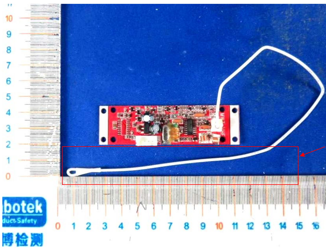
MIC RX Antenna
