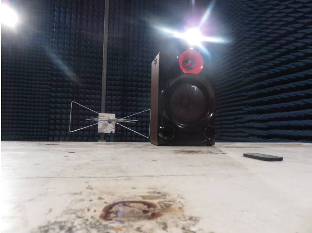
Photo of Radiation Emission Test
