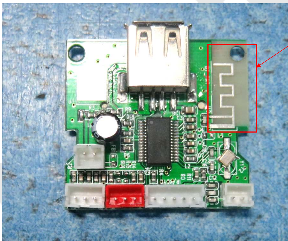
BT Antenna
