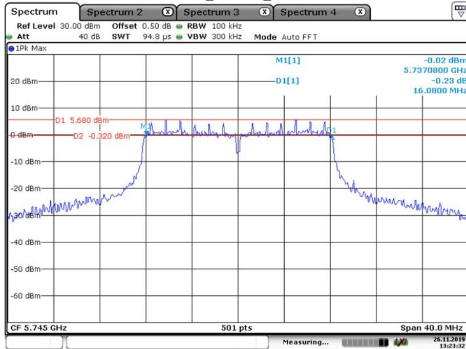
5.8G_802.11 a_Low
