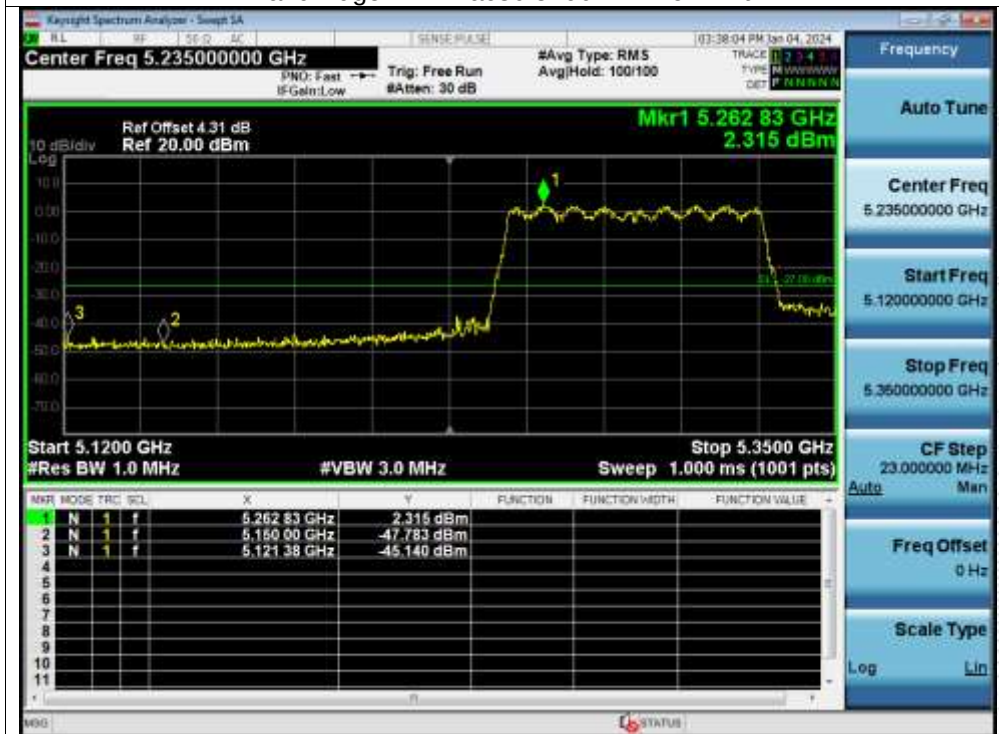
Band Edge NVNT ac80 5290MHz Low Ant1
