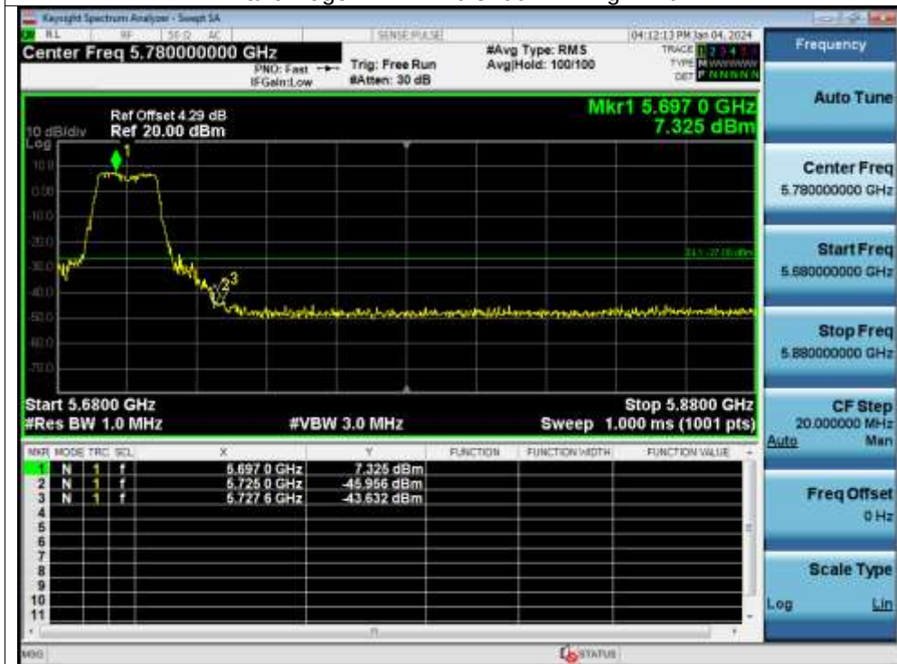
Band Edge NVNT n20 5700MHz High Ant1
