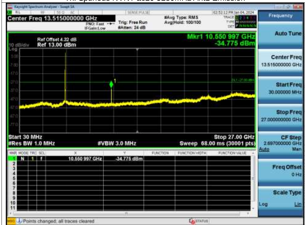
Tx. Spurious NVNT ac20 5280MHz Ant1 Emission
