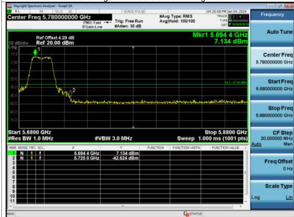
Band Edge NVNT ac20 5700MHz High Ant1
