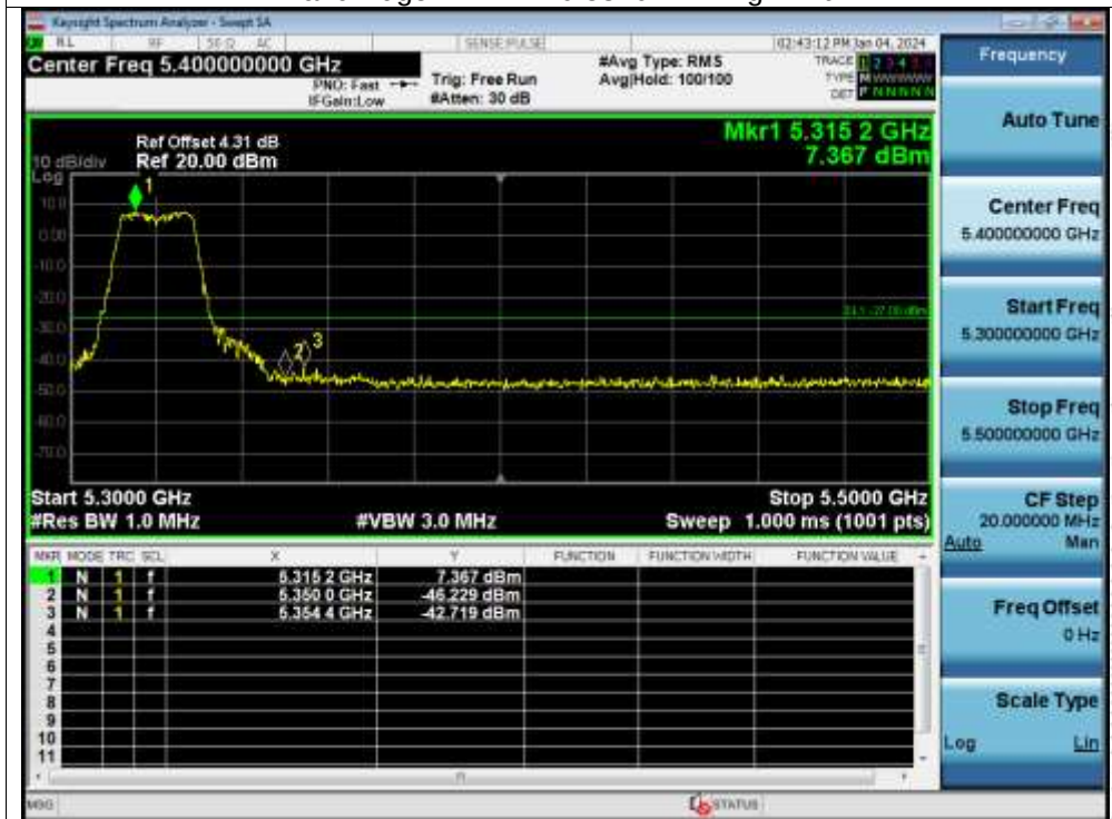
Band Edge NVNT n20 5320MHz High Ant1
