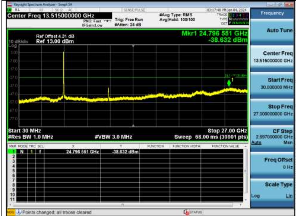
Tx. Spurious NVNT n40 5310MHz Ant1 Emission
