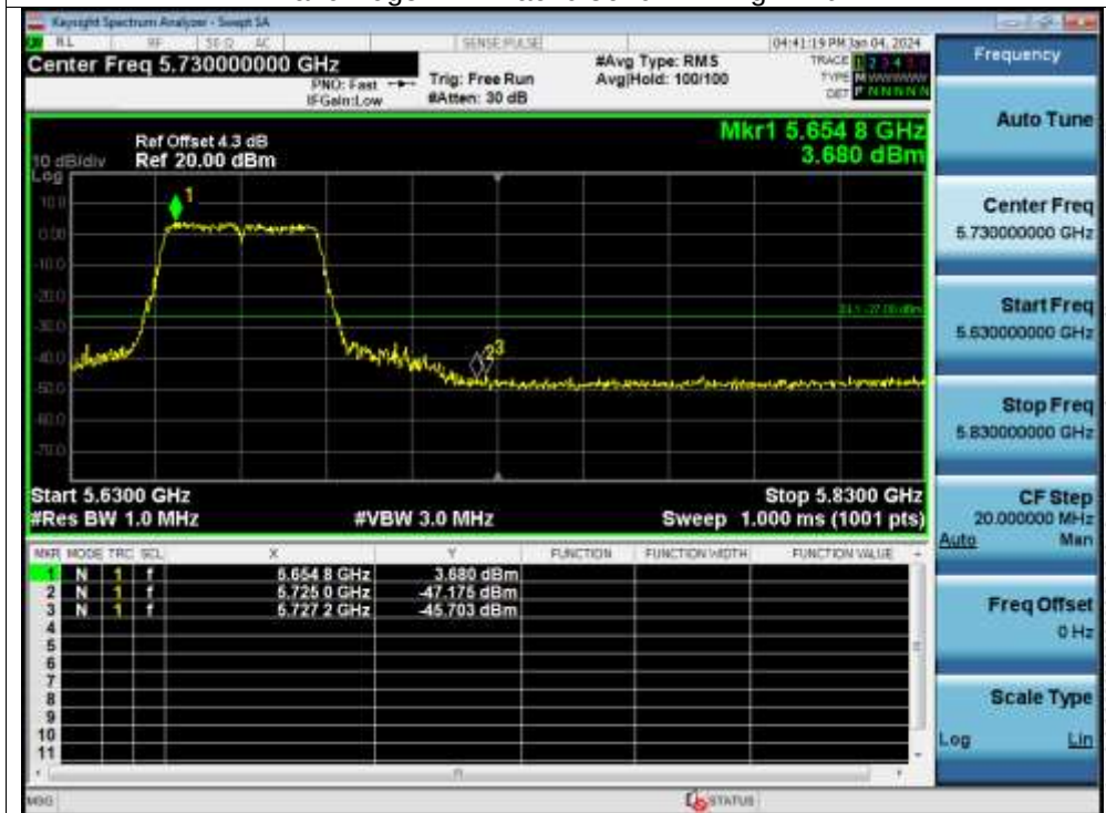
Band Edge NVNT ac40 5670MHz High Ant1
