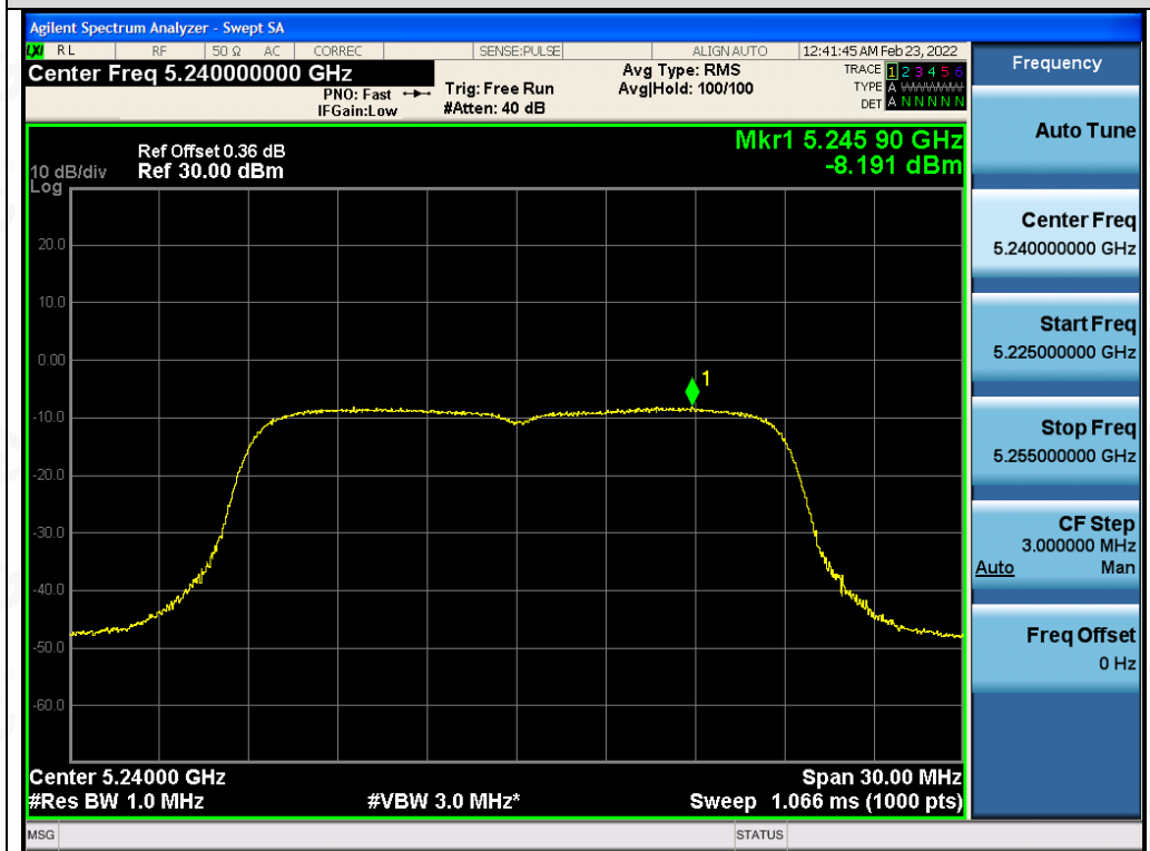
Test_Graph_802.11n20_ANT2_5240_MCS0_PSD
