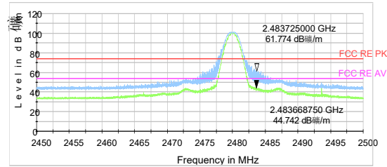
Bluetooth LE ((S=8) Channel 39 Peak+Average
