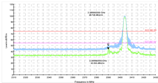
Bluetooth LE ((S=8) Channel 0 Peak+ Average
