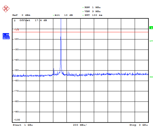
LTE Band 4 5MHz CH-Low 1GHz~3GHz
