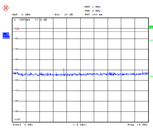
LTE Band 4 5MHz CH-Low 3GHz~18GHz
