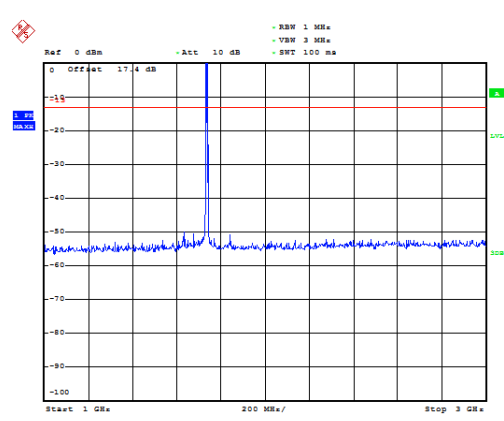
LTE Band 4 5MHz CH-Middle 1GHz~3GHz
