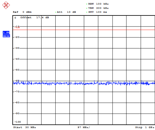
LTE Band 4 5MHz CH-Low 30MHz~1GHz
