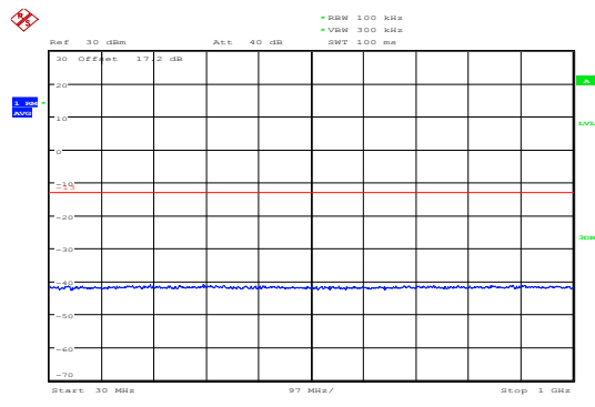
LTE Band 4 1.4MHz CH- Middle 30MHz~1GHz
