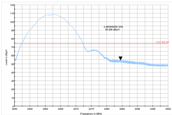
802.11b-Channel 11 Peak
