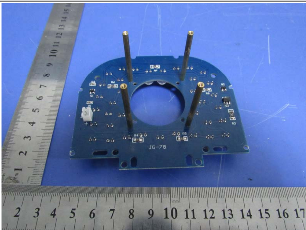
EUT LED Light - Rear View
