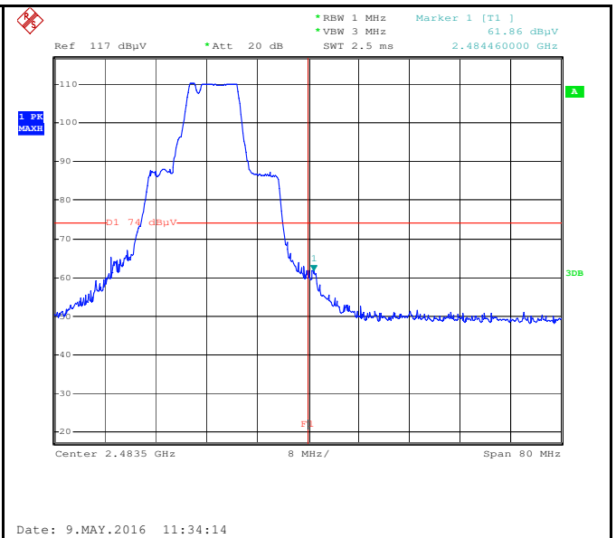
Band Edge, Right Side (Peak)
