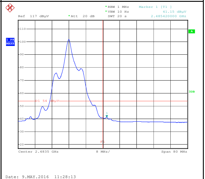
Band Edge, Right Side (Average)
