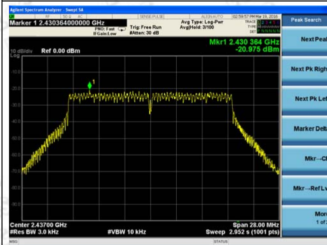
802.11n HT20_Middle Channel / 2437MHz
