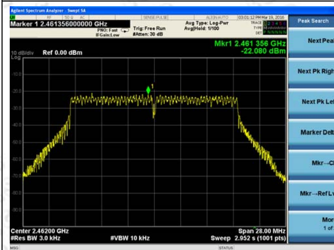
802.11n HT20_High Channel / 2462MHz
