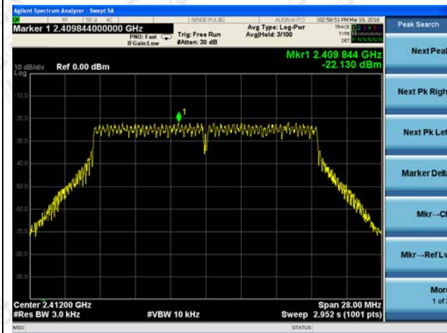
802.11n HT20_Low Channel / 2412MHz
