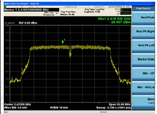
802.11n HT40_Low Channel / 2422MHz
