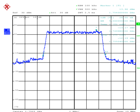
Modulation: QPSK
