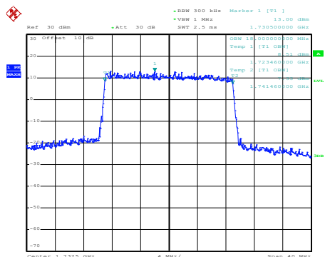
Modulation: 16QAM
