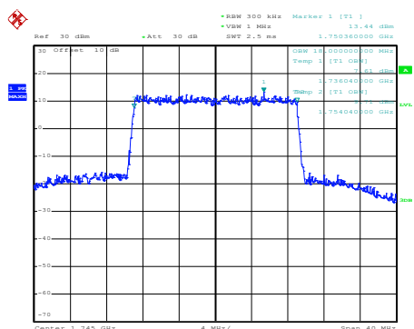
Modulation: 16QAM
