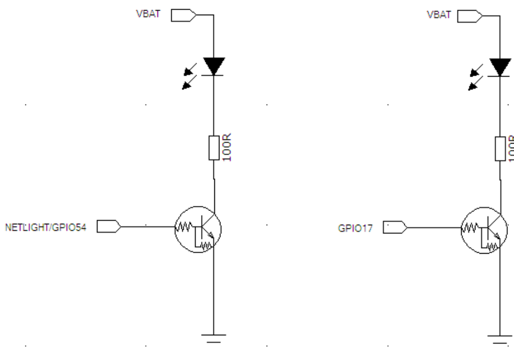
Figure 3-10 LED Circuit
