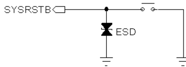
Figure 3-2: System Reset
