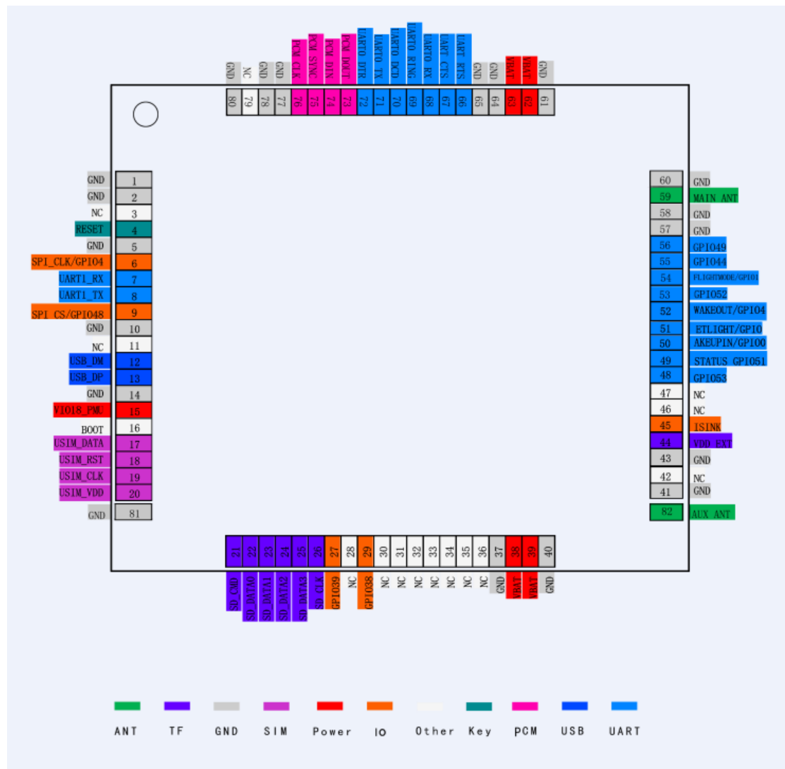
Figure 2-1: L306 PIN View
