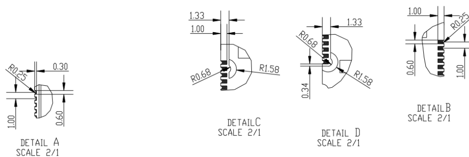
Figure 2-3 Package SIZE
