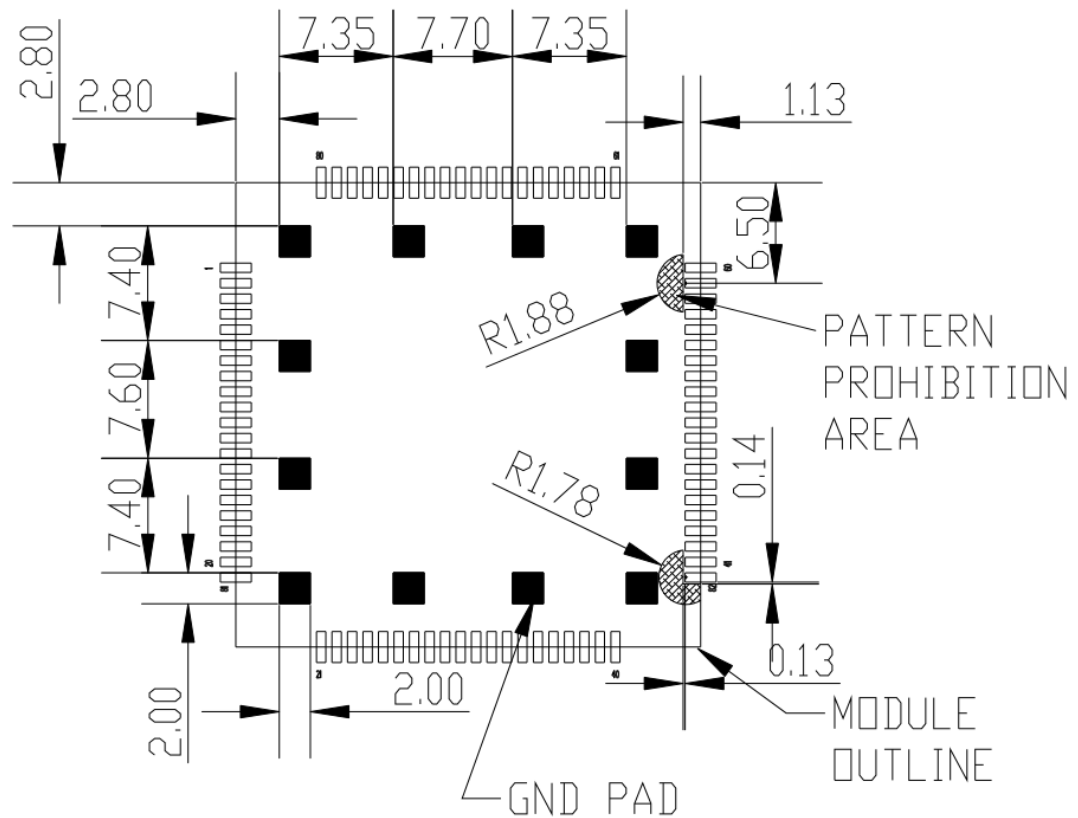
Figure 2-4 Recommend pad
