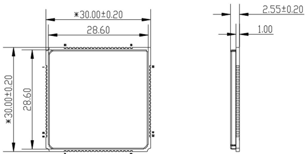
Figure 2-2 Module SIZE
