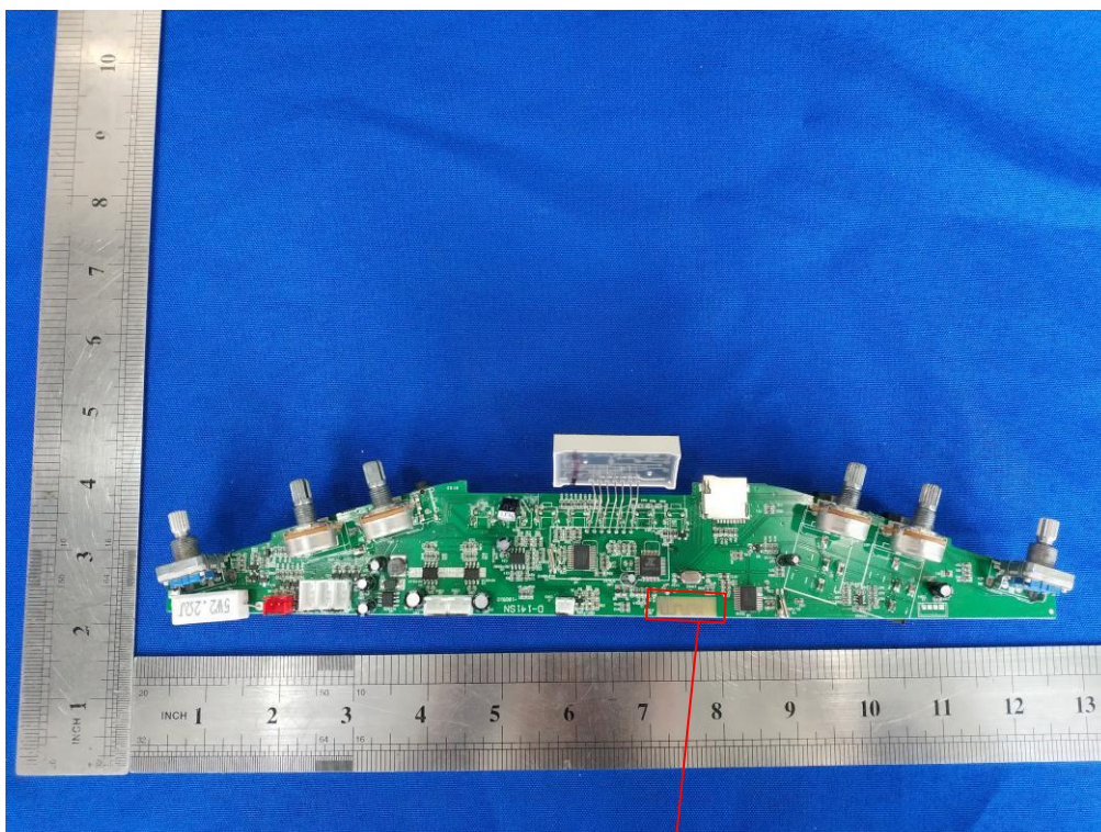
BT:PCB antenna
