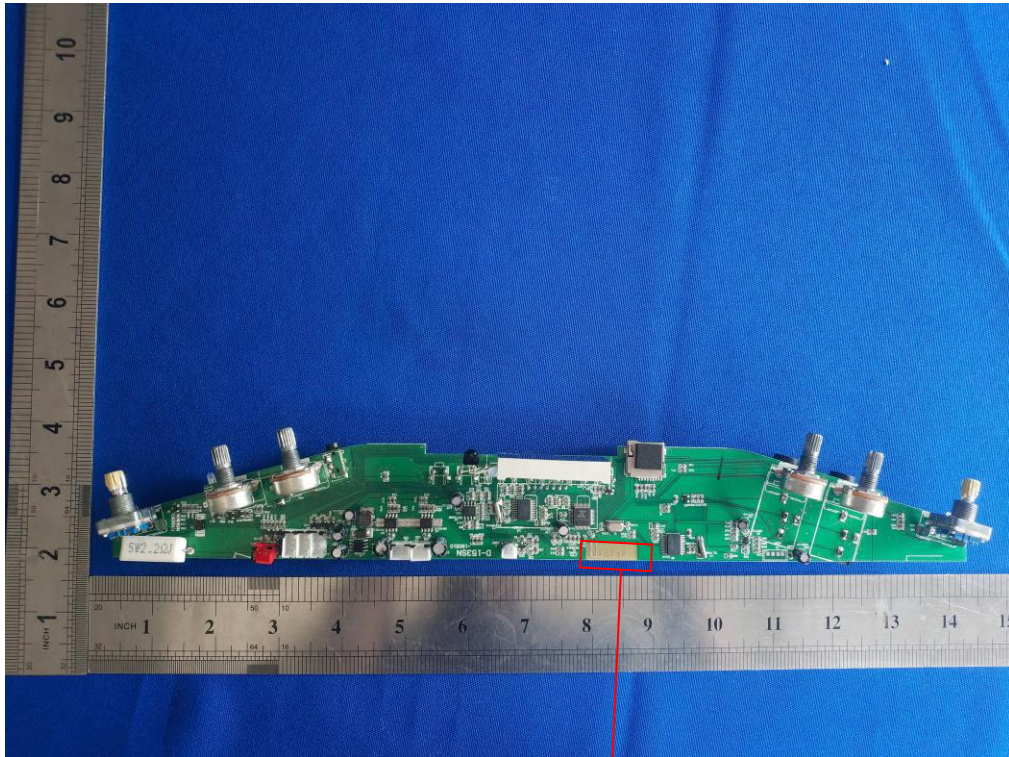
BT:PCB antenna
