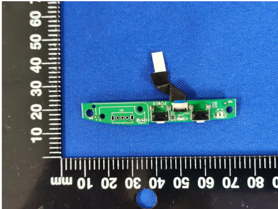
BOARD TOP VIEW
