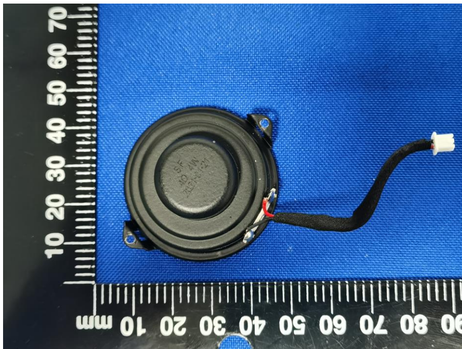
SPEAKER REAR VIEW
