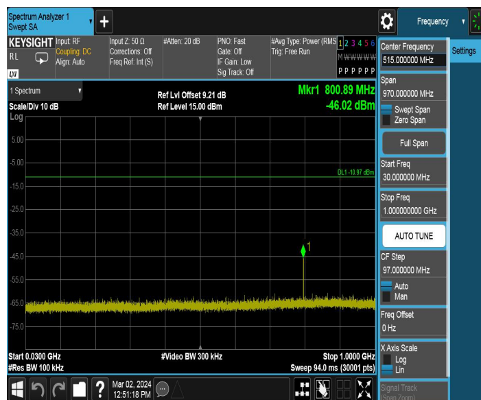
BLE_1M_Ant1_2402_30~1000
