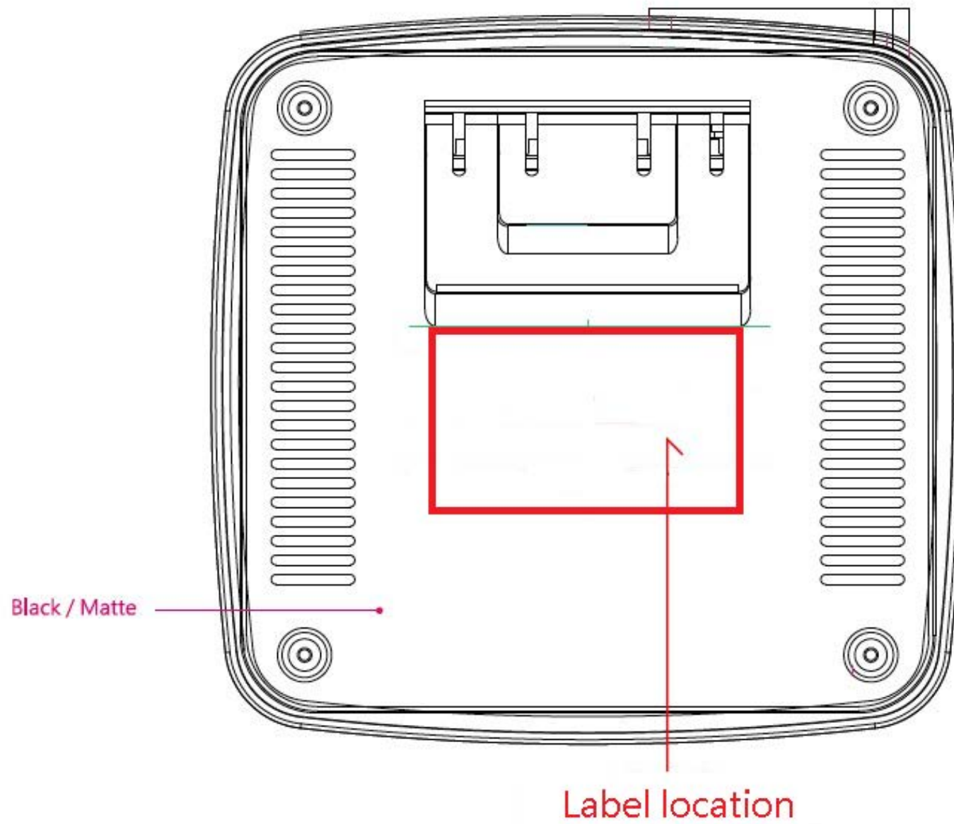
Bottom View
