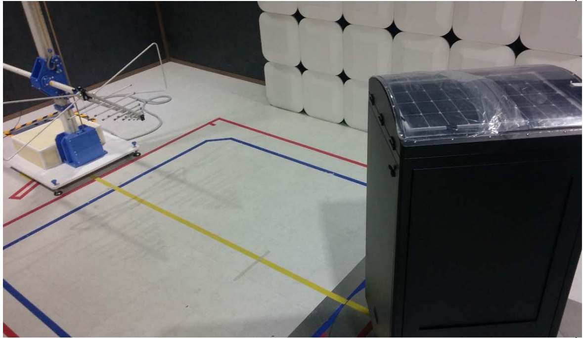
Test Setup Photo of Radiated Measurement (below 1000MHz)
