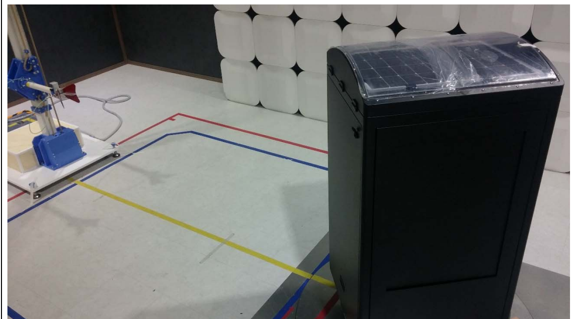
Test Setup Photo of Radiated Measurement (Above 1GHz)
