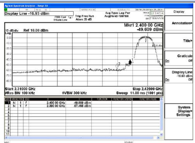
Channel 1 / 2412 MHz
