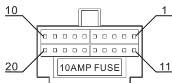
DETAIL A SHOWN FROM PIN VIEW
