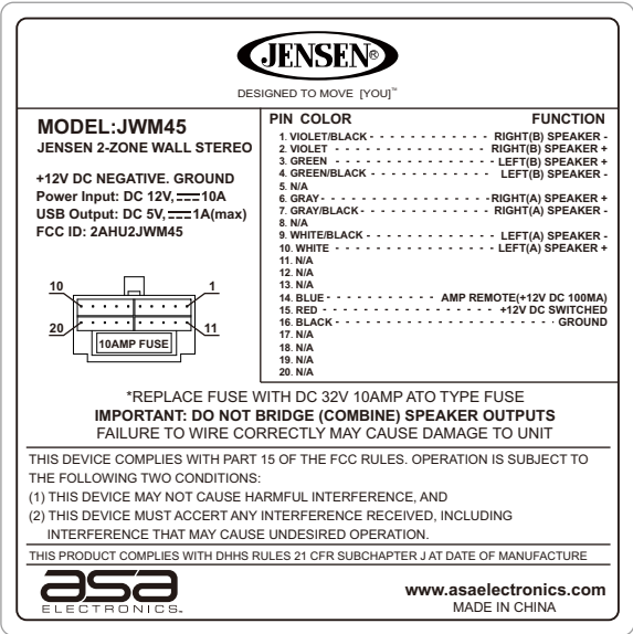
1. MODEL PLATE(80x80mm) P/N: 508W100A0G
