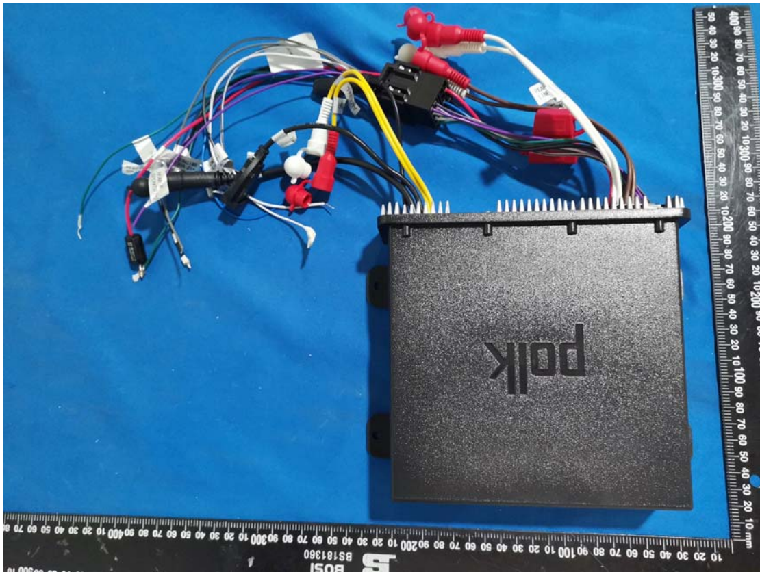
Tuner/Amp Module
