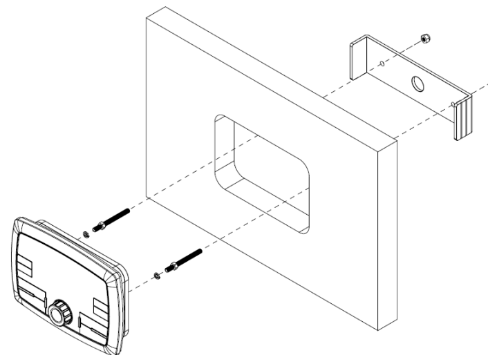
Bracket Mount
