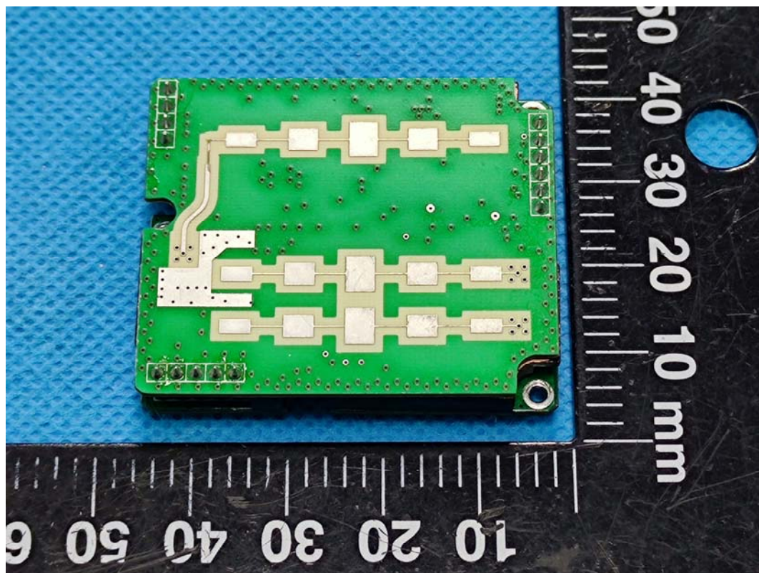
Right Sensor
