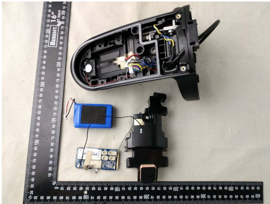
UNCOVER VIEW 3
