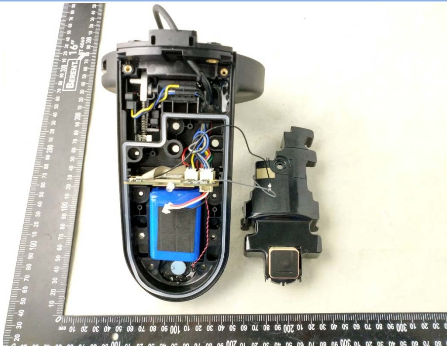
UNCOVER VIEW 2
