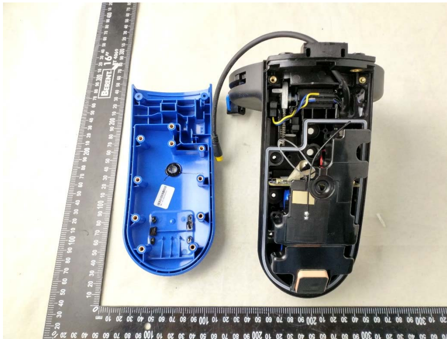
UNCOVER VIEW 1
