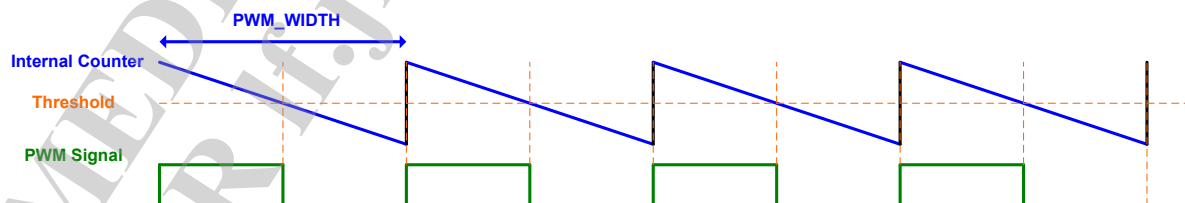
Figure 43. PWM waveform.
