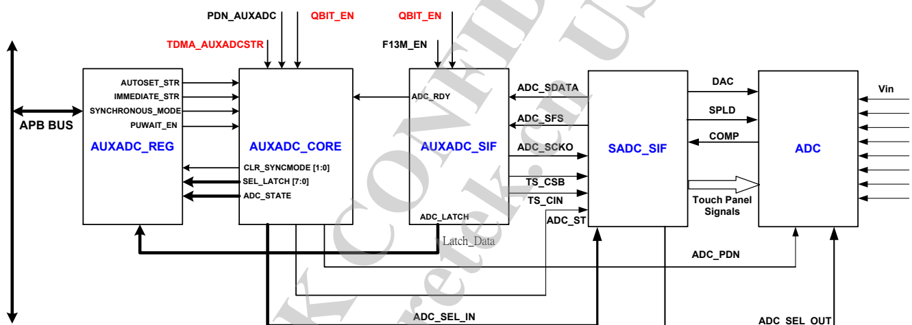
Figure 38. AUXADC architecture
