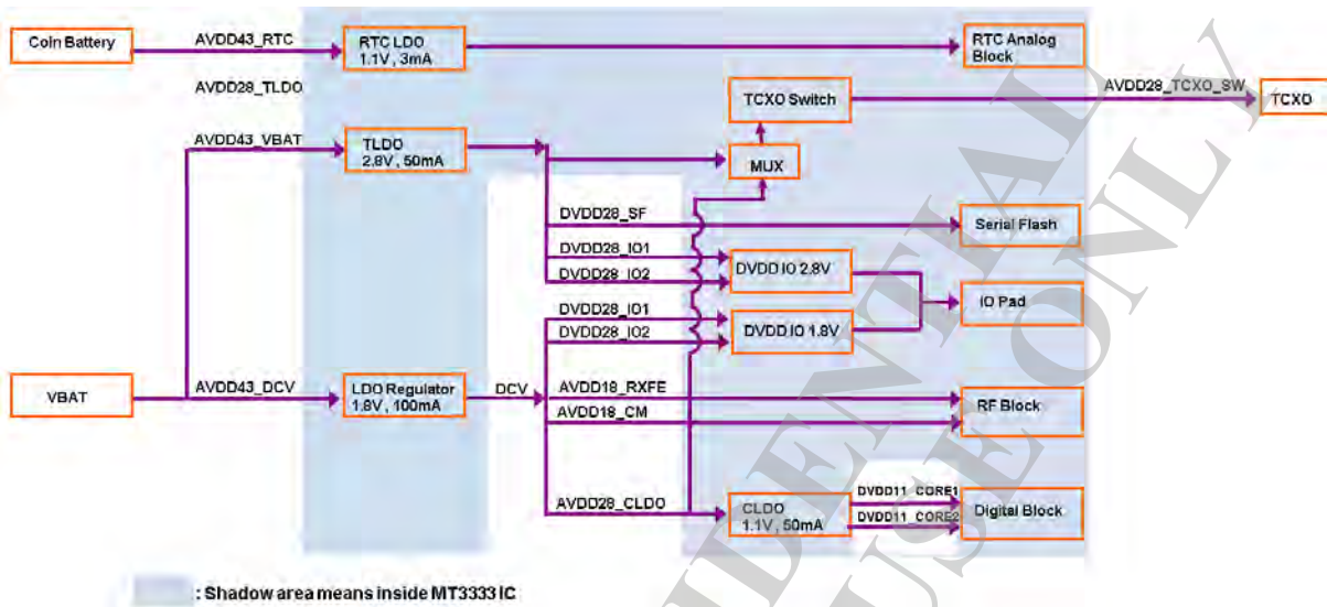
Figure 55. Power supply connection (low cost)
