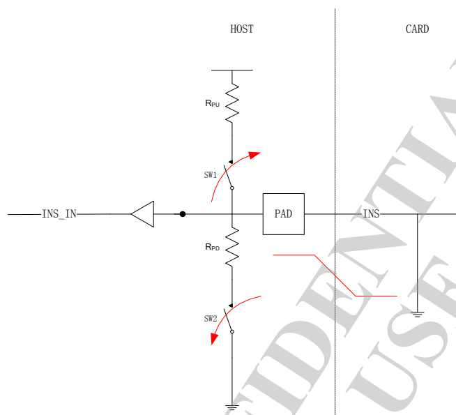
Figure 46. Card detection for SD memory card
