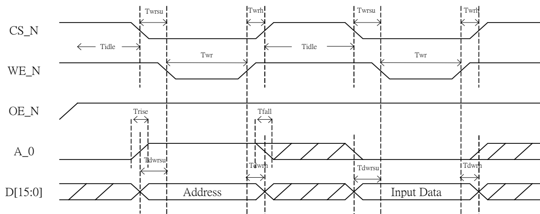
Figure 25. eHPI write cycle timing diagram
