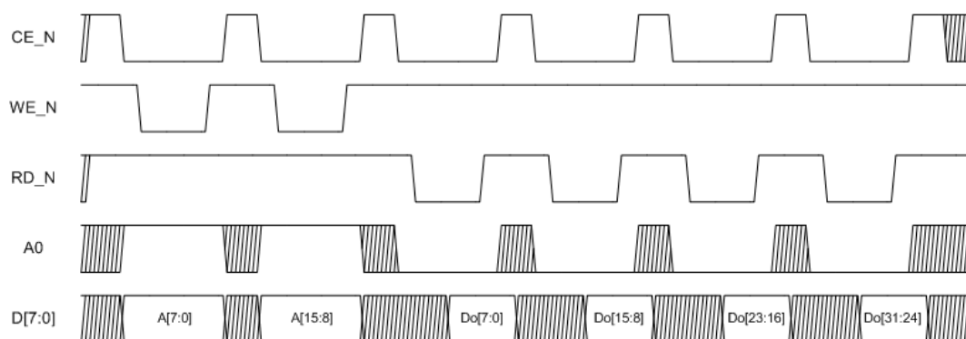
Figure 19. eHPI8 burst write access (data port)
