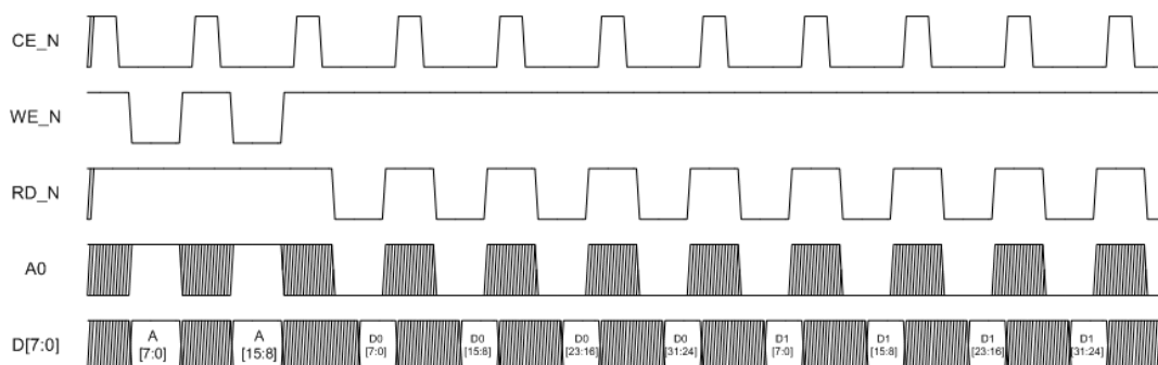
Figure 20. eHPI18 burst read access (data port)
