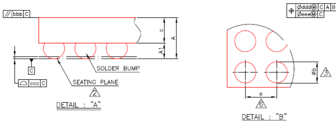
Figure 7. MT5931 WLCSP POD (b)
