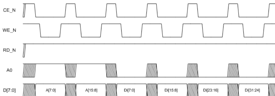
Figure 17. eHPI8 single write access
