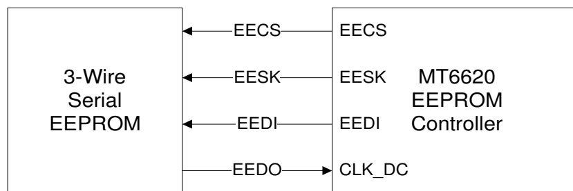
Figure 29. EEPROM interface connection
