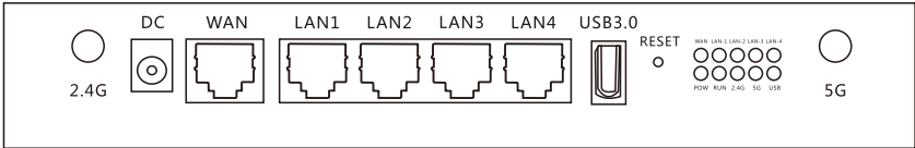
Figure- 1 Router Physical Interfaces
