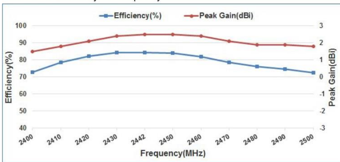
7-3. 3D Efficiency vs. Frequency
