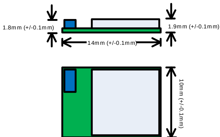
Figure 9-3 External Dimension
