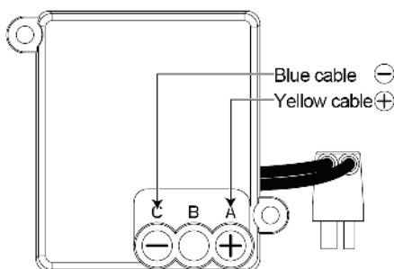
The back size of receiver
