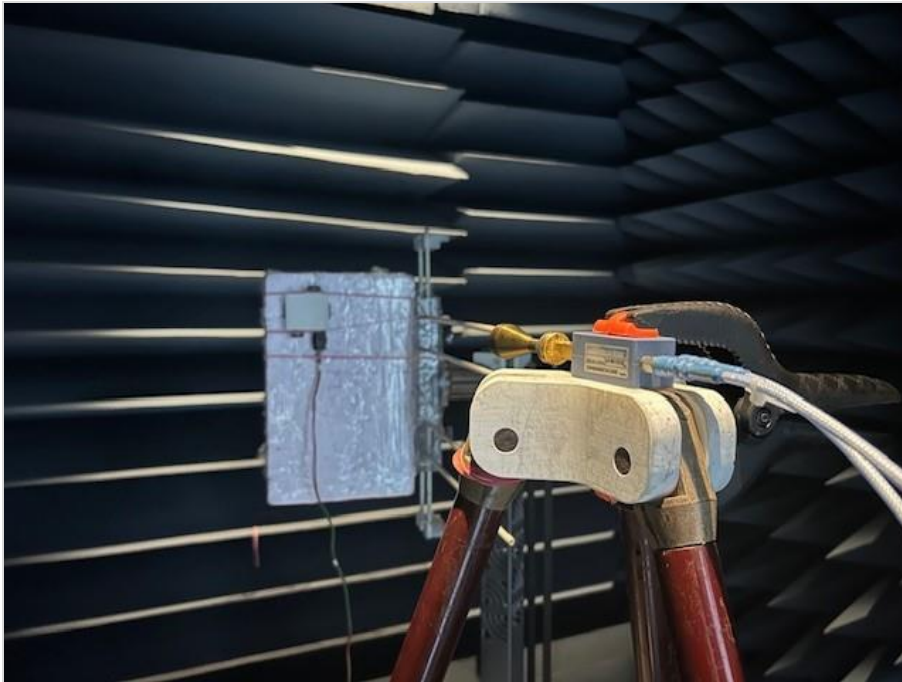
Photograph 1: EUT test setup in the fully anechoic chamber-2
