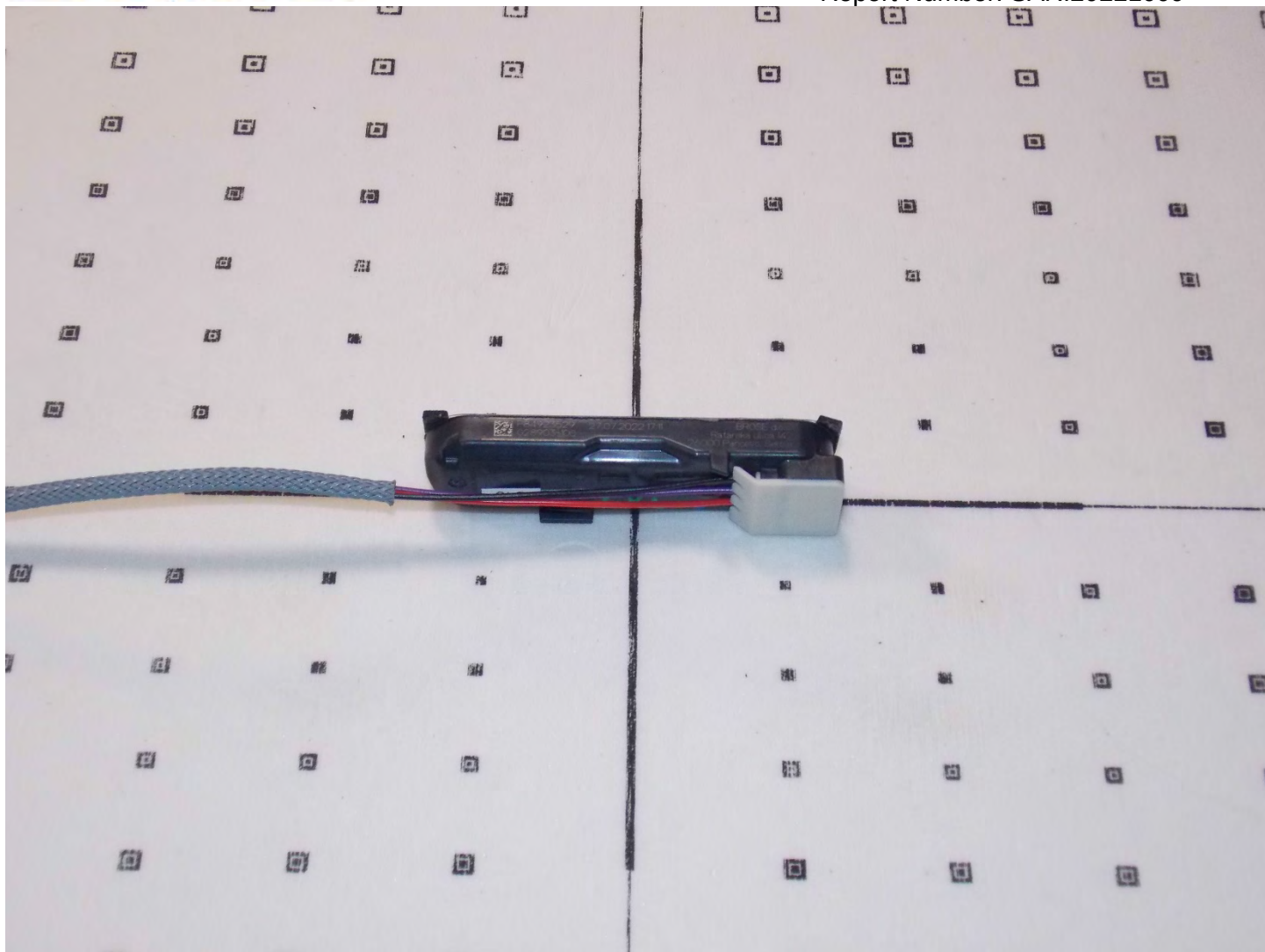
Test Position Right 4.6 mm Gap
