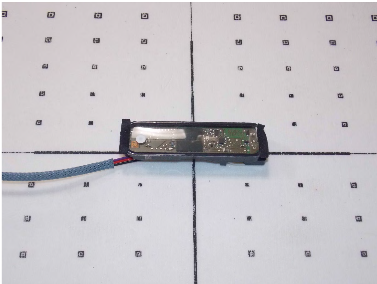
Test Position Front 4.6 mm Gap
