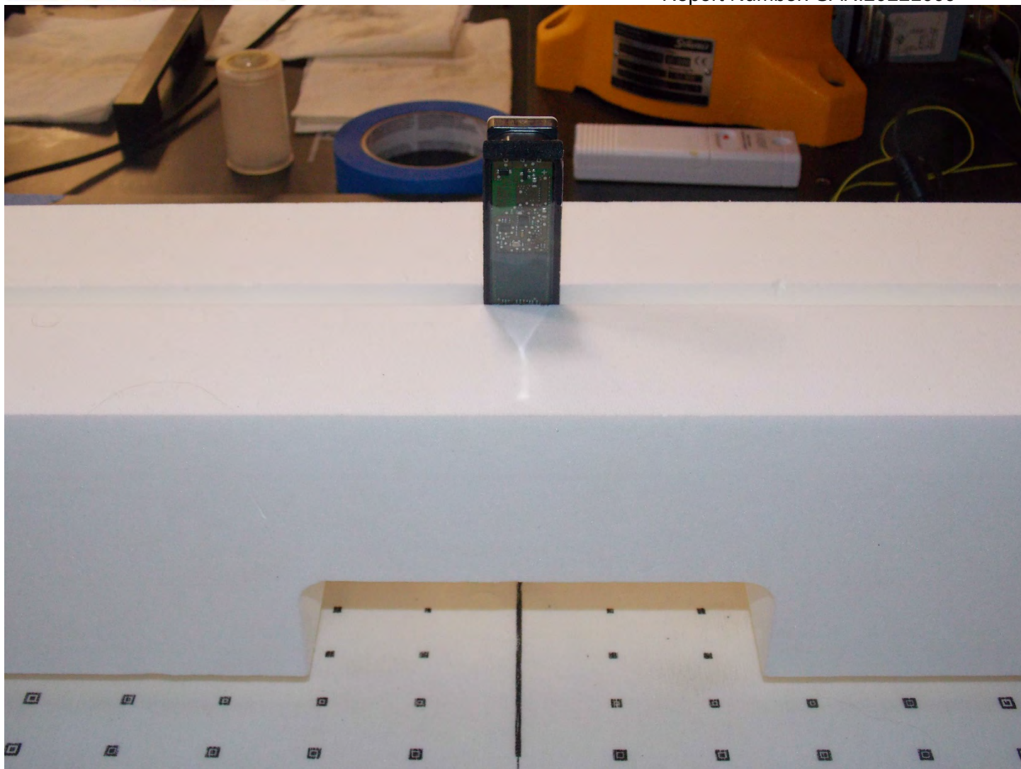
Test Position Top 4.6 mm Gap
