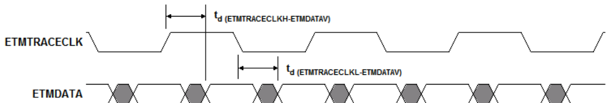
Figure 8-17. ETMDATA Timing
