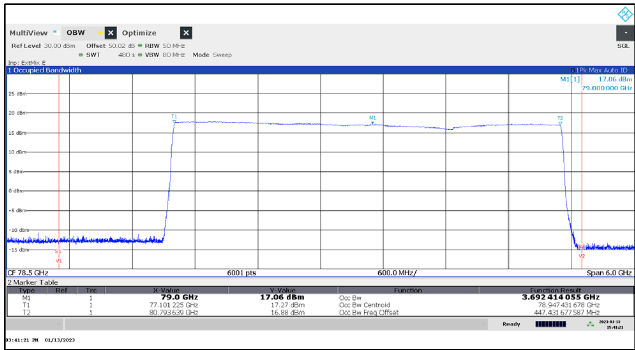
Plot 4: 99% Bandwidth
