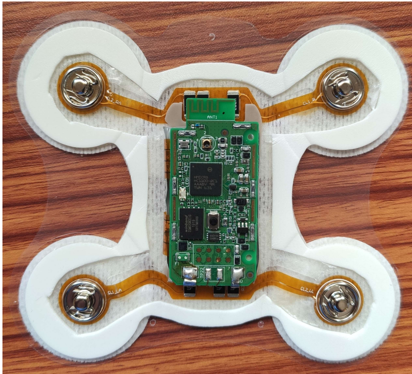
Photo 1: Internal Photo Without Shield
