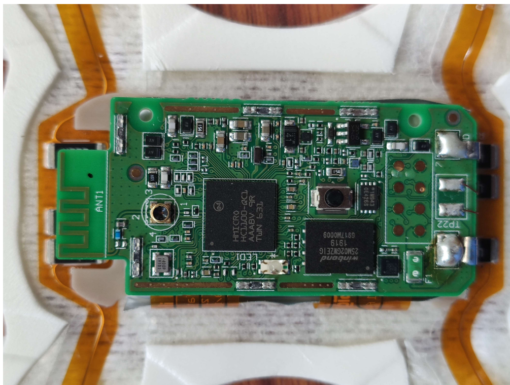
Photo 2: Internal Photo Rigid PCB
