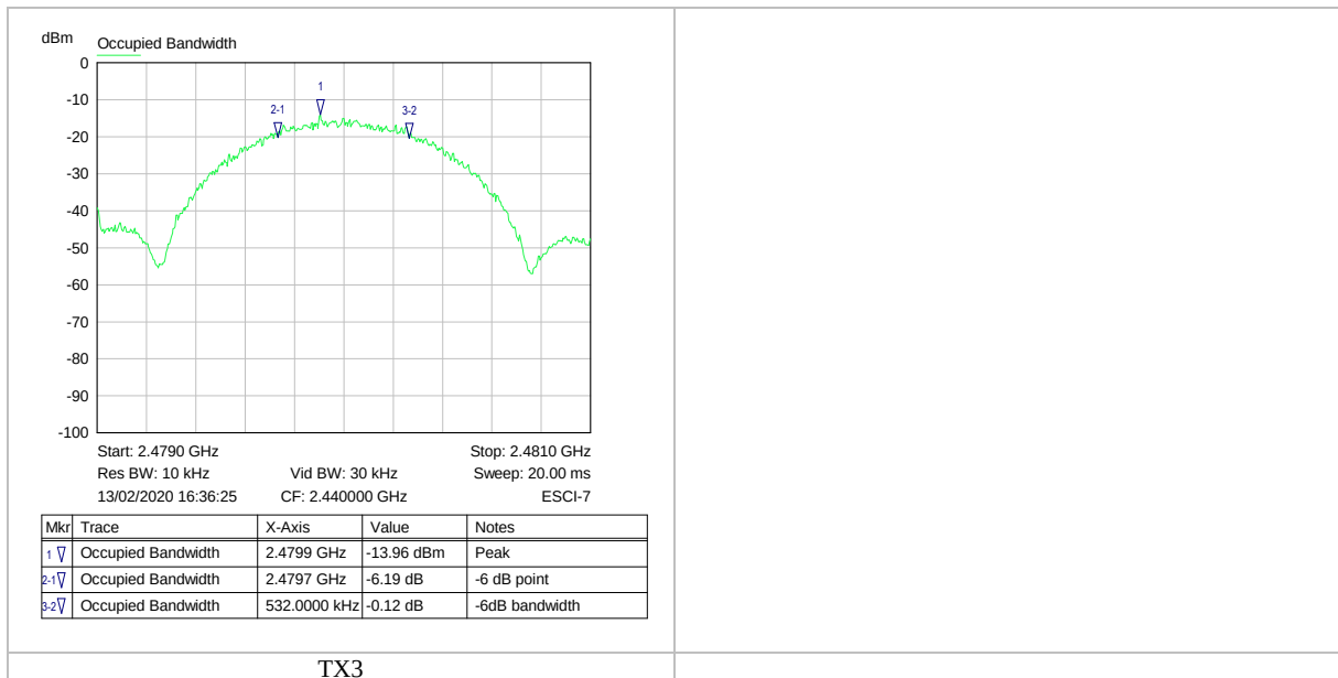
Figure 2: Occupied Bandwidth
