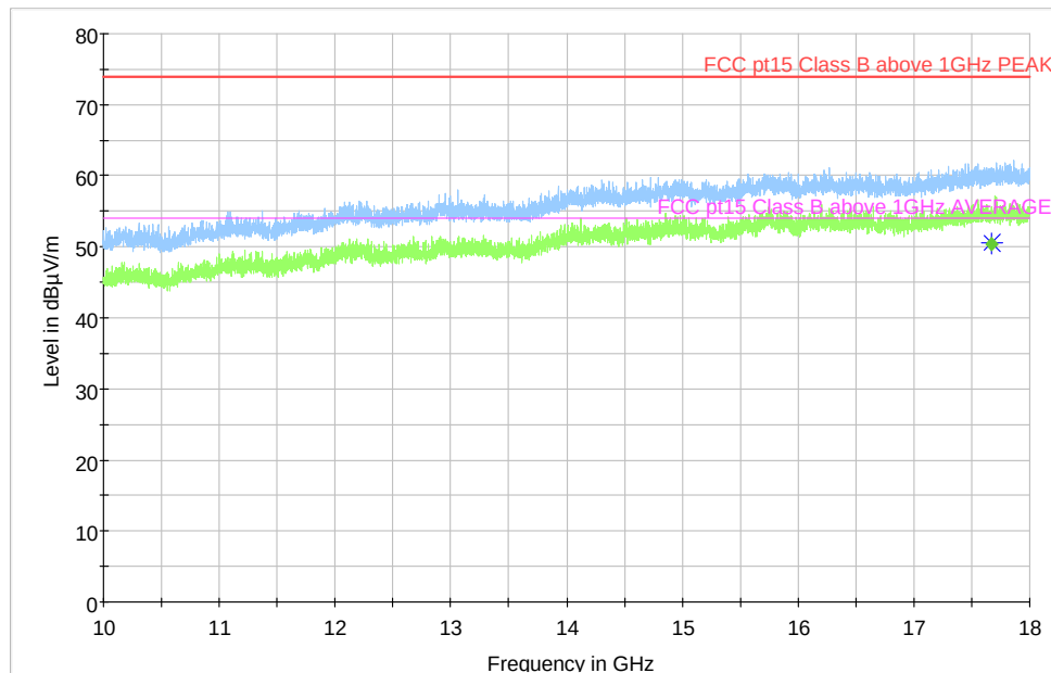
10 to 18GHz, Middle Channel, 2440MHz, X Orientation
