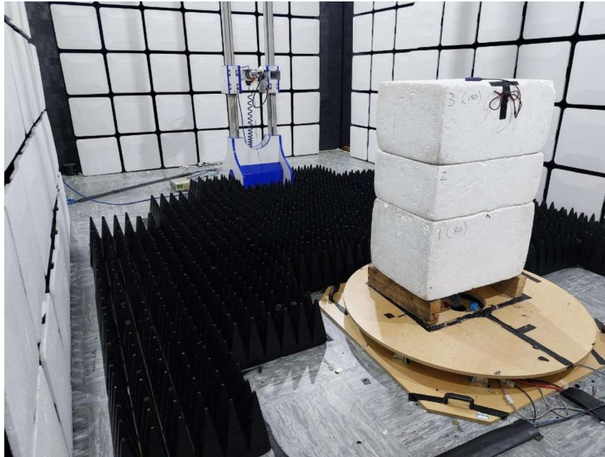
Figure 52 – Test Setup 8 GHz to 18 GHz
