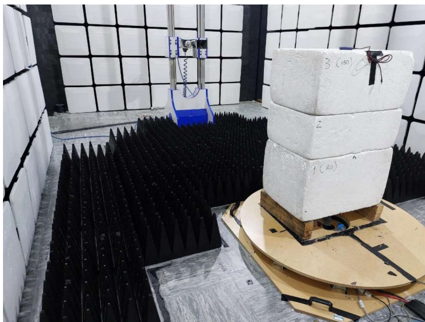
Figure 51 – Test Setup 1GHz to 8 GHz
