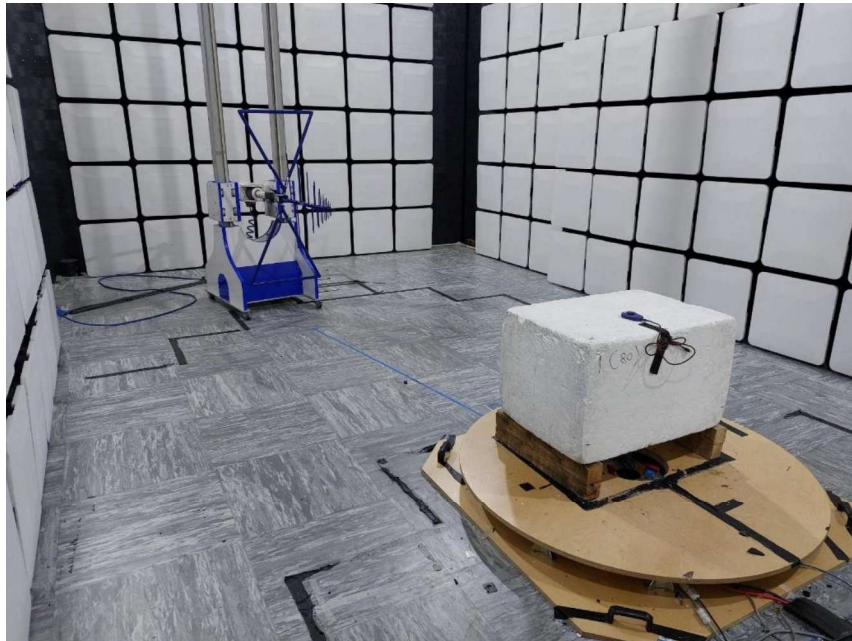
Figure 50 – Test Setup 30MHz to 1GHz
