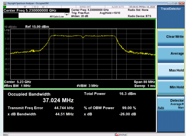
Channel 5230MHz
