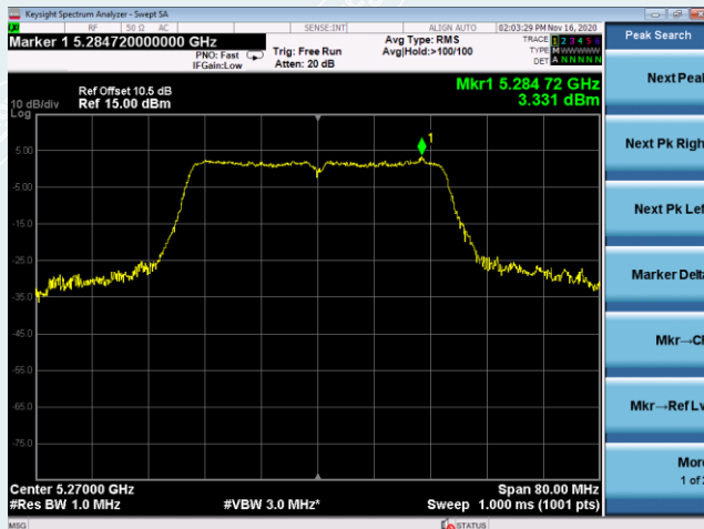
Channel 5270MHz
