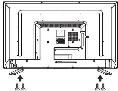
Screws x 4
