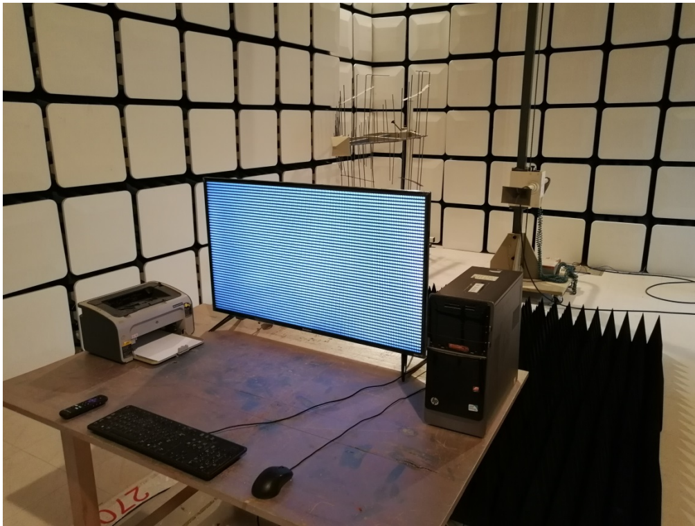
Radiated Measurement Photo 1000~6000MHz
