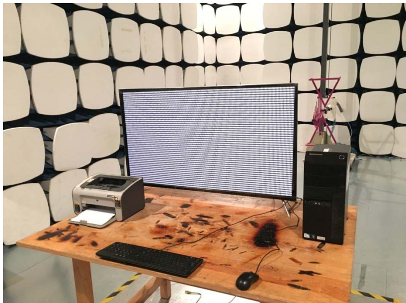
Radiated Emission
